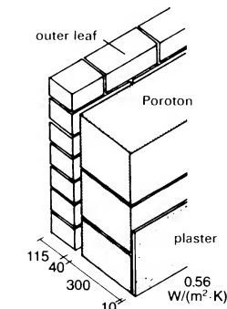
⑯ Poroton (clay insulating block) cavity wall 0.56 W/(m 2 ·K)
